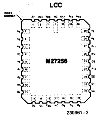
Figure 2. Pin Configurations
